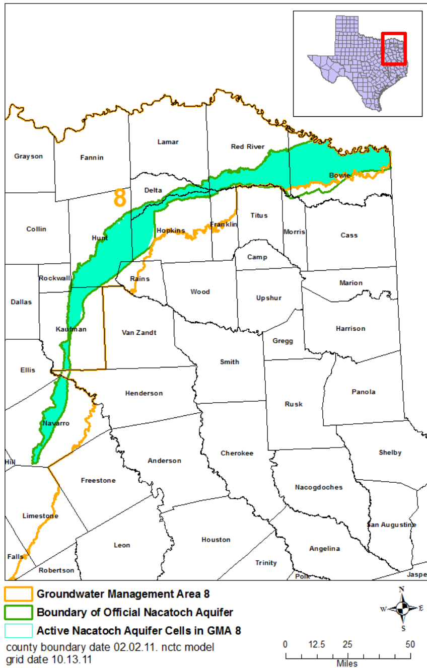
FIGURE 11. EXTENT OF THE GROUNDWATER AVAILABILITY MODEL FOR THE NACATOCHE AQUIFER USED TO ESTIMATE TOTAL RECOVERABLE STORAGE FOR THE NACATOCHE AQUIFER IN GROUNDWATER MANAGEMENT AREA 8.
